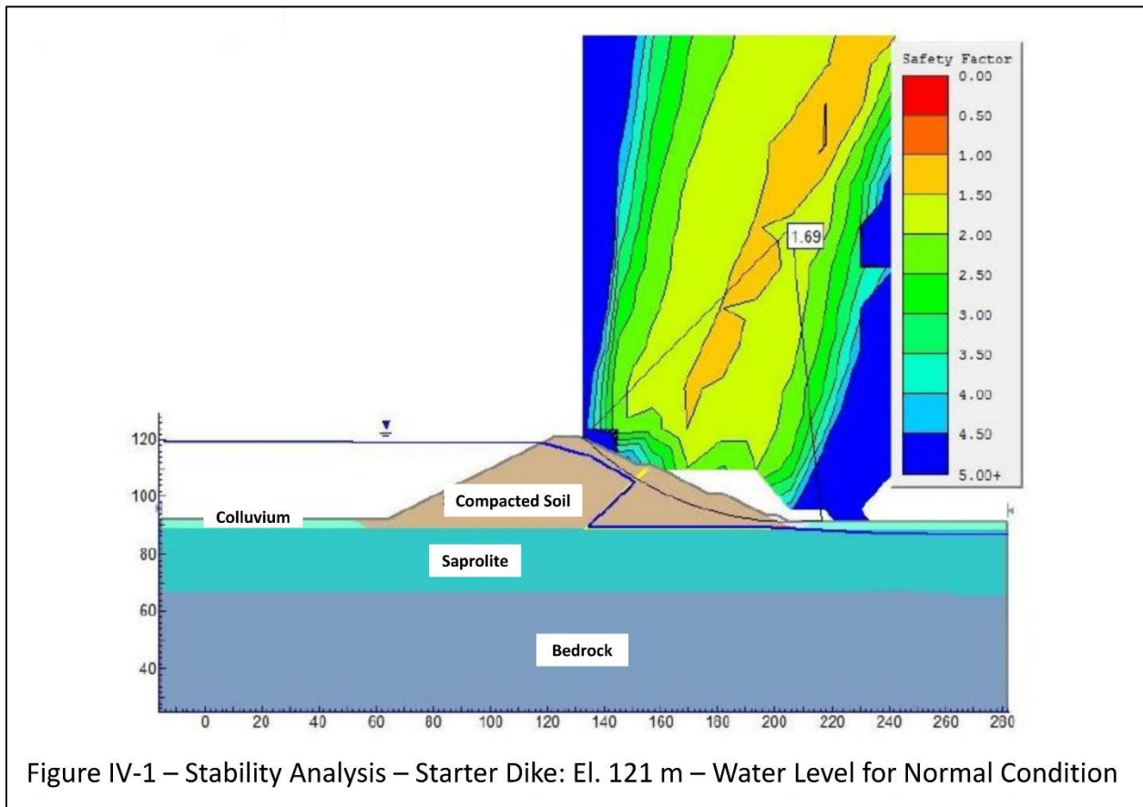
Figure 12a. The starter dike would have a factor of safety of 1.69, where the factor of safety is the minimum ratio of the shear resistance to the shear stress, considered over all possible failure surfaces. The calculated factor of safety exceeds the minimum value of 1.50 that is required by Brazilian tailings dam regulations (ABNT, 2017). However, the factor of safety was calculated only for the static condition and not for the dam response to seismic acceleration, contrary to the same tailings dam regulations that require design to withstand the Maximum Credible Earthquake (ABNT, 2017). No stability analyses have been provided for the final dike (see Fig. 8). Note the role of the internal drainage system (see Fig. 8) in lowering the water table within the starter dike. Figure from VOGBR (2016a) overlain with English labels.
