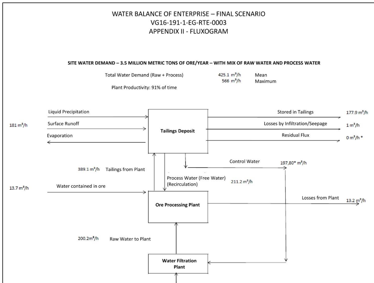
Figure 10. The mixture of tailings and water would be thickened to a 53% solids content before export to the tailings deposit. However, the addition of 181 cubic meters of water from the catchment for every 389.1 cubic meters of water from the ore processing plant would give the mixture of tailings and water an effective solids content of 43%, which is within the range for conventional tailings management with no thickening. The addition of catchment water to the tailings deposit is the opposite of the current practice of constructing diversion canals around the tailings deposit in order to prevent the entry of catchment water so as to reduce the water stored behind the tailings dam. Because of the use of cyanide in the ore processing plant, the recirculation of water from the tailings deposit has the potential to increase the concentrations of antimony, arsenic and mercury in the water with each passage through the ore processing plant. Portion of figure from VOGBR (2016b) overlain with English labels.
