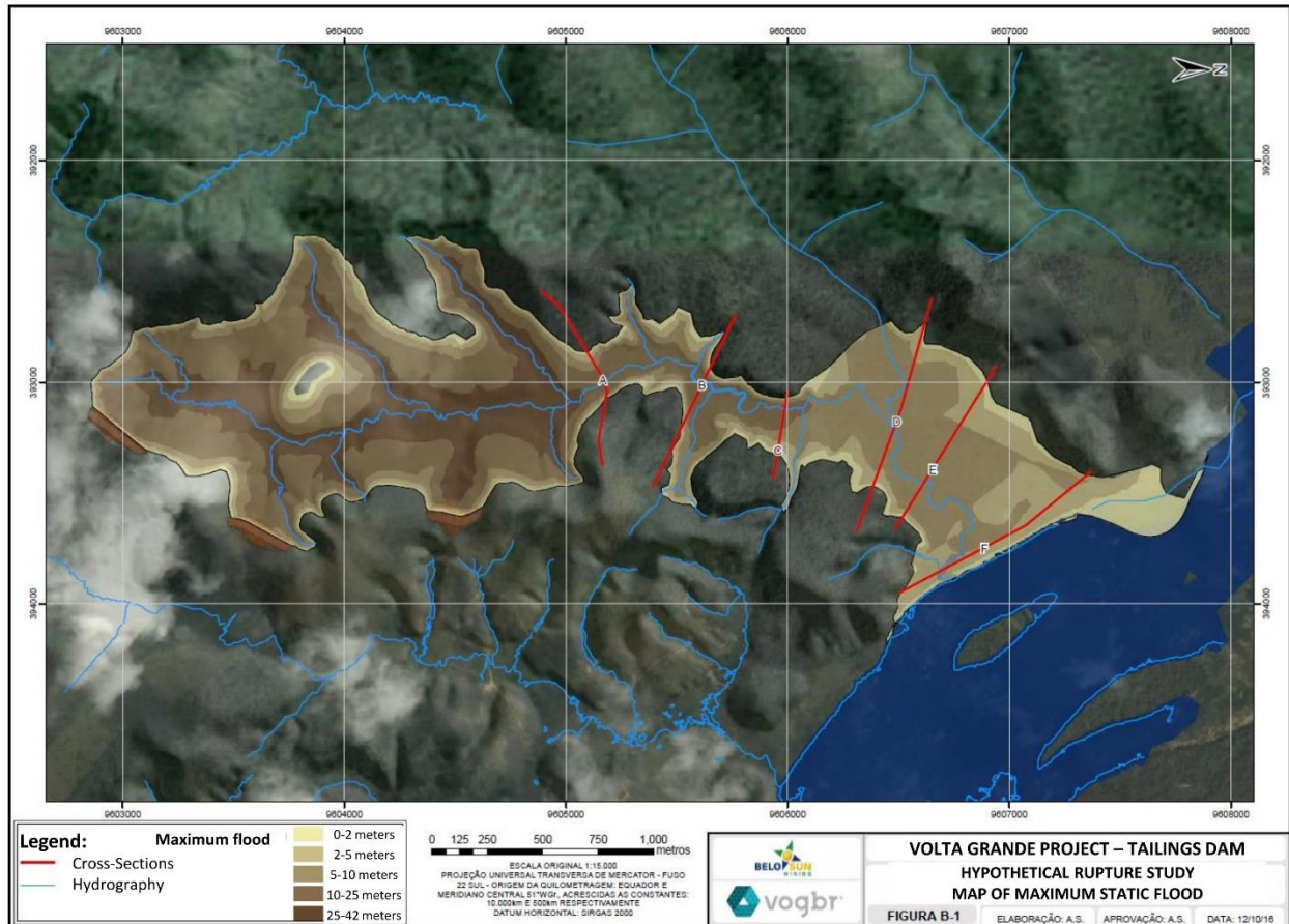
Figure 14. The dam break analysis was flawed in that it assumed that the tailings flood would cease when the tailings reached the Xingu River (Brandt Meio Ambiente, 2016). Cross-section A is the edge of the tailings dam (compare with Fig. 3 for location, but note difference in north arrows). The figure is overlain with English labels and comes from a report that was not available to the author.
